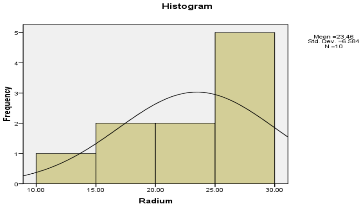
Fig 6: Chart of Activity concentration of ^{226}\text{Ra} in sediment
