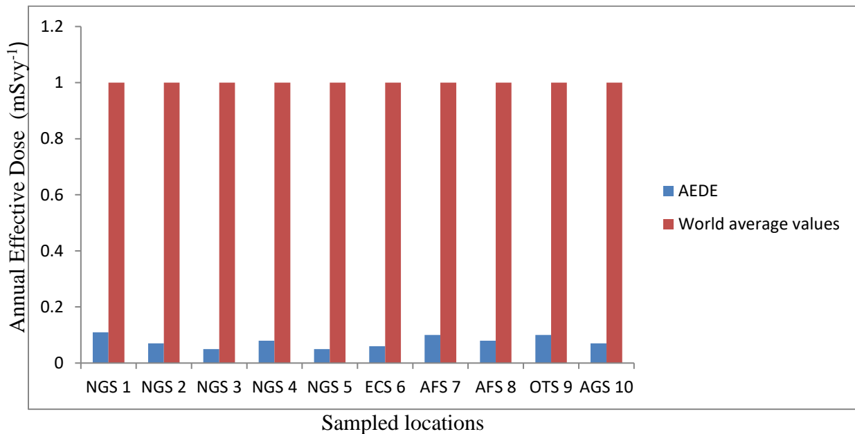
Fig 9: Comparison of Annual Effective Dose (mSvy -1 ) in sediment with World average values in all the locations
