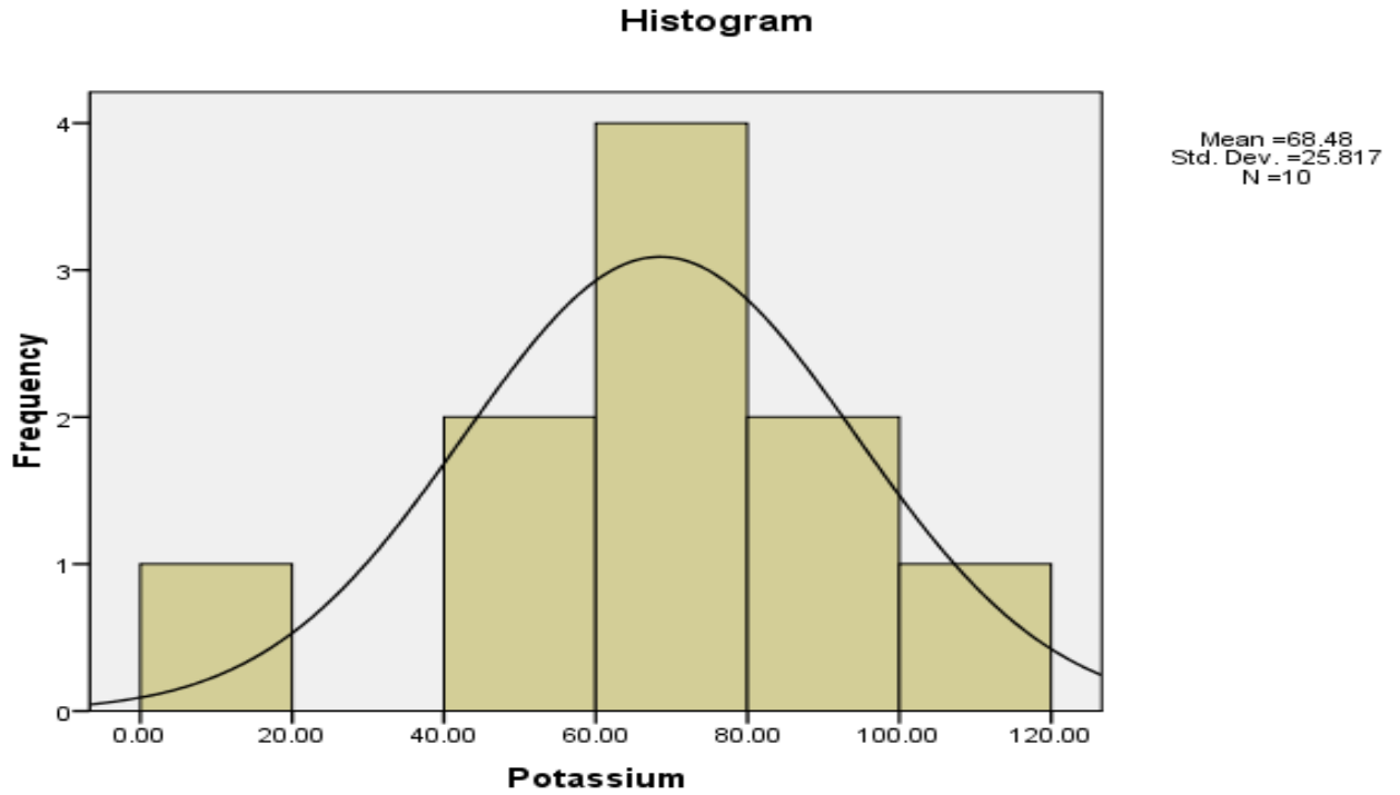
Fig 5 Chart of Activity concentration of ^{40}\text{K} in sediment
